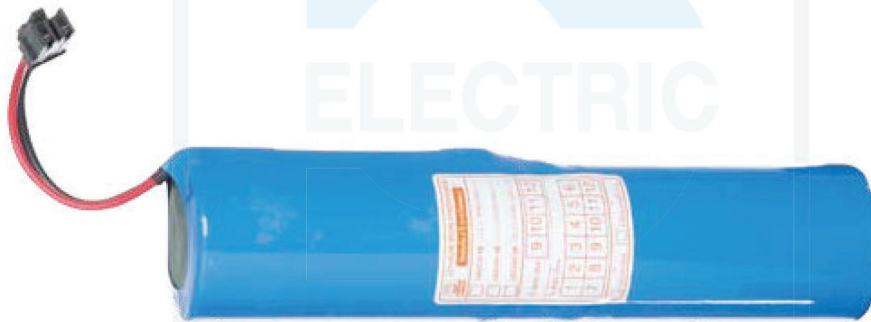
Model: LB3260-2B Nominal voltage: 3.2 V Nominal capacity: 12000 mAh For DYNO emergency light model: LFG-12P4T, PWD-IP65-12P4T
